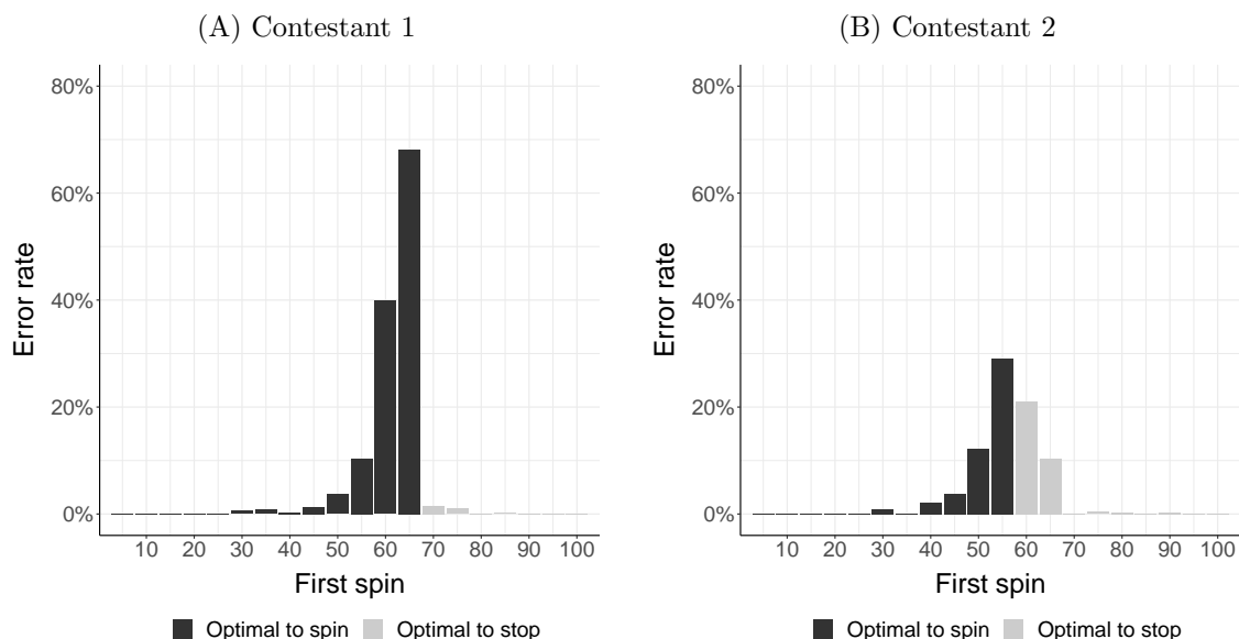
Figure 2: Deviations from the SPNE
